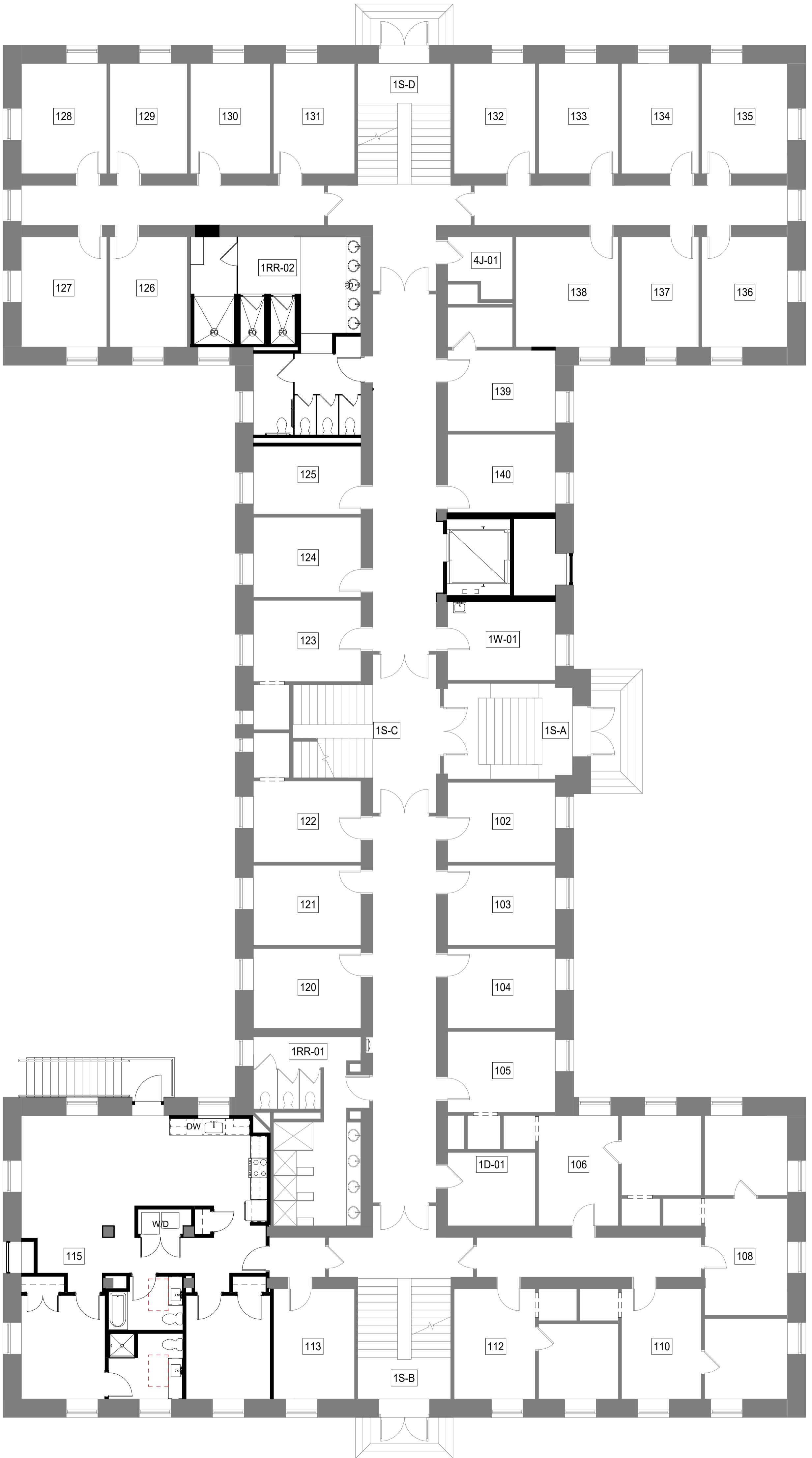
1 LEVEL 1 ROOM NUMBERING 1/8" = 1'-0"
