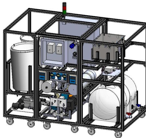
CAD Model
